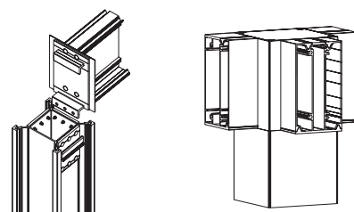
Mullion and intermediate transom connection
