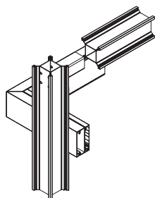
Mullion and transoms connection
