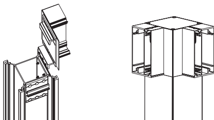
Mullion and transom connection
