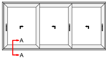
FRONT VIEW Όψη
