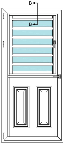
Όψη FRONT VIEW
