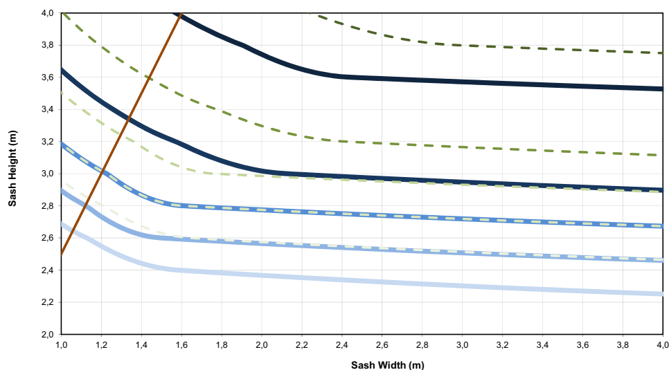
Maximum Panel Dimensions For Given Wind Pressure
