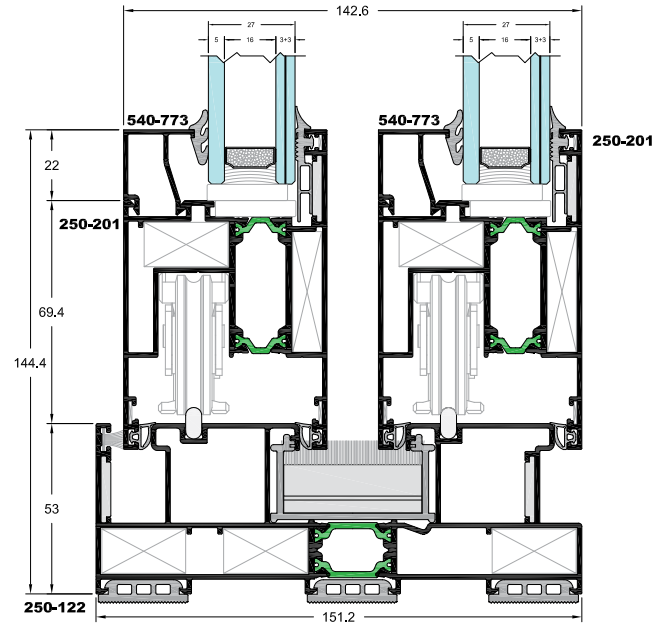
ΟΔΗΓΟΣ ΕΠΑΛΛΗΛΟΥ OVERLAPPING RAIL
